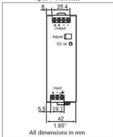
Fig. 20-1 Front view
