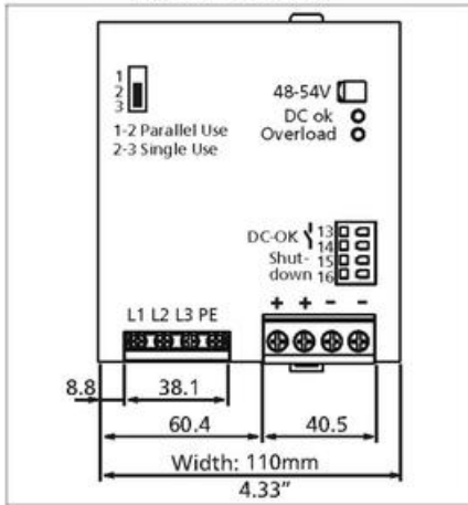
Fig. 22-1 Front view
