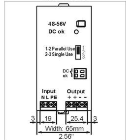
Fig. 20-1 Front view
