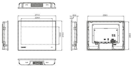
Panel Cut-out Dimensions: 260 x 201.5 mm (10.24" x 7.93")
