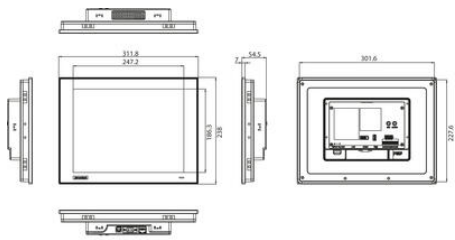
Panel Cut-out Dimensions: 302.5 x 228.5 mm (12.1" x 9.14")
