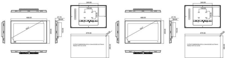
Panel Cut-out Dimensions: 479.30 x 300.30 mm (18.87" x 11.82")
