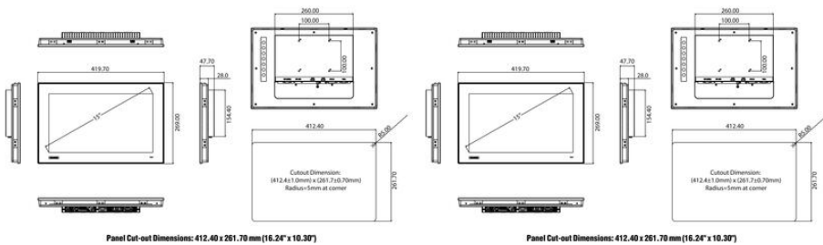
Panel Cut-out Dimensions: 412.40 x 261.70 mm (16.24" x 10.30")
