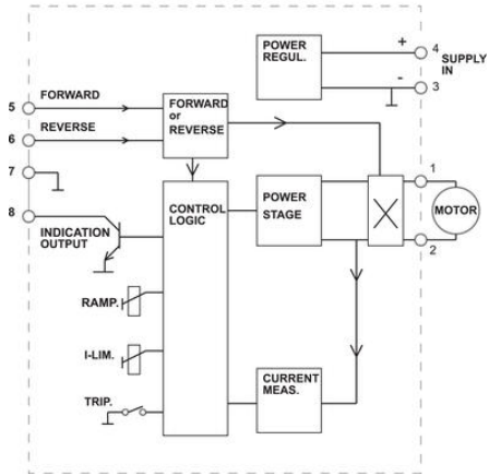
EM-140A BLOCK DIAGRAM
