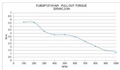
Torque Curve
