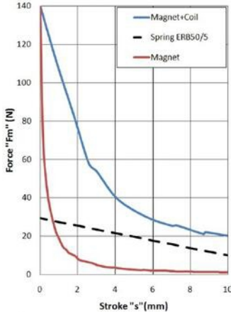
Force-Stroke Curve (F-S)
