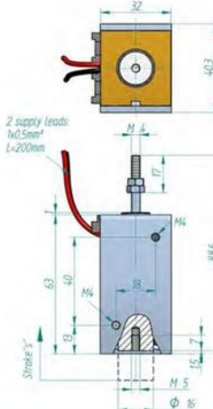
Locked solenoid
