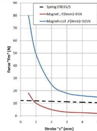
Force-Stroke curve(F-S)
