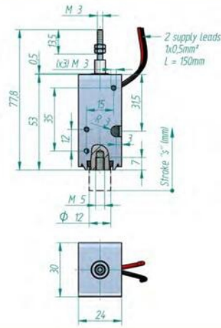
Solenoid locked
