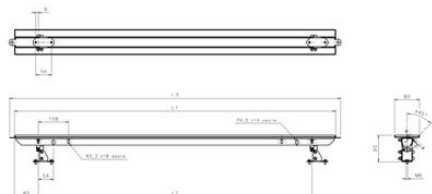
Models 600 to 1900, including ST-DM stand alone bracket mounting kit
