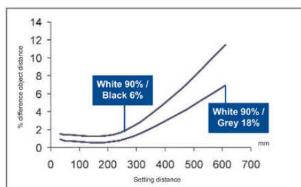
60 ... 600 mm Wall-hanging
