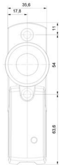
Magnet unit
