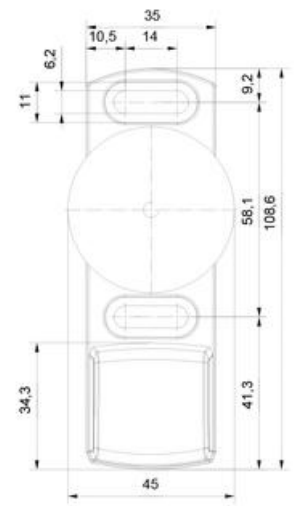
Anchor plate
