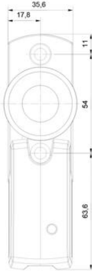
Magnet unit
