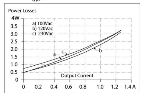
Fig. 8-2 Losses vs. output current at 12V, typ.
