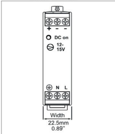
Fig. 20-1 Front view
