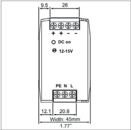
Fig. 20-1 Front view
