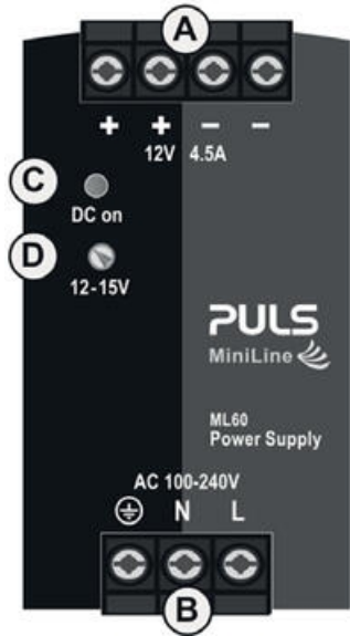
Fig. 10-1 Front side
